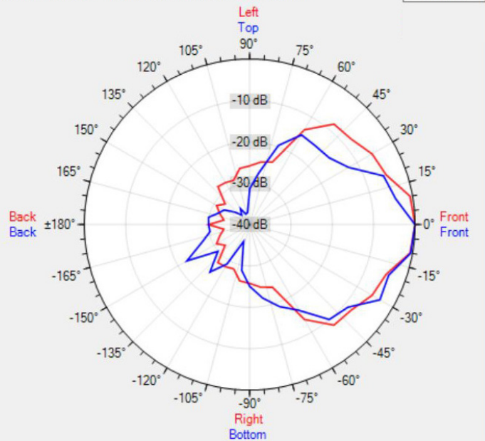
Data Shown: MASK8 (Apart Audio) Display Parameters: Frequency: 8000Hz (1/24th Octave)
