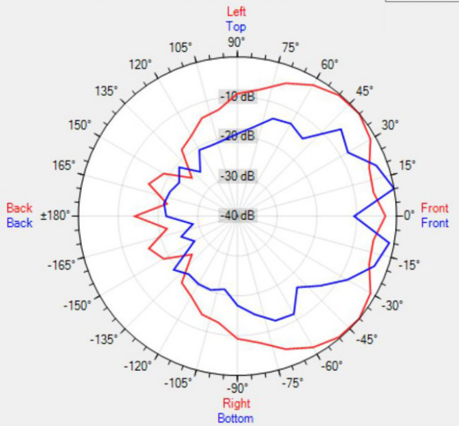
Data Shown: MASK8 (Apart Audio) Display Parameters: Frequency: 4000Hz (1/24th Octave)
