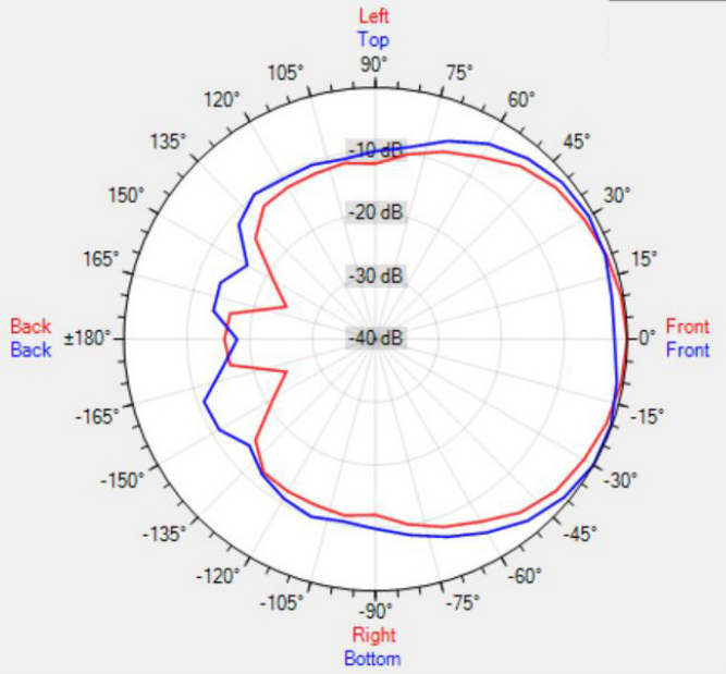
Data Shown: MASK8 (Apart Audio) Display Parameters: Frequency: 1000Hz (1/24th Octave)
