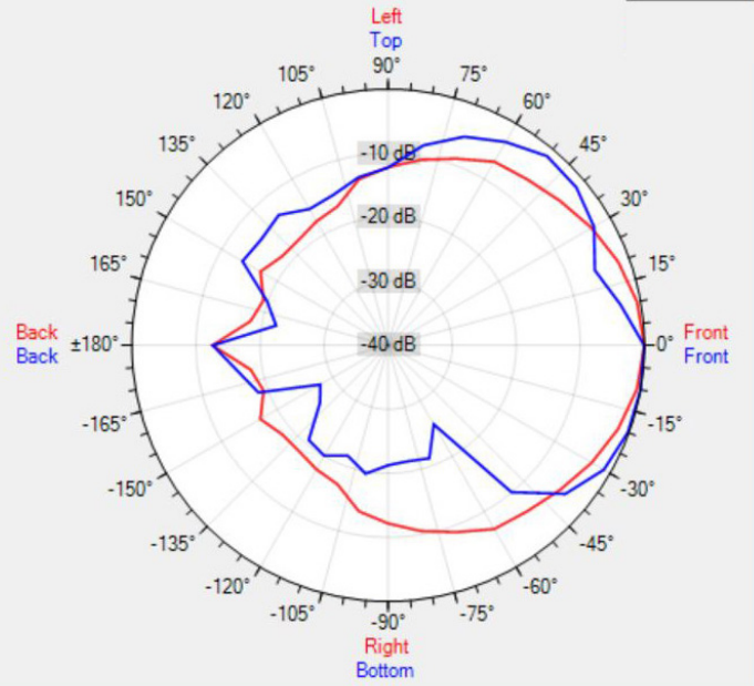
Data Shown: MASK8 (Apart Audio) Display Parameters: Frequency: 2000Hz (1/24th Octave)
