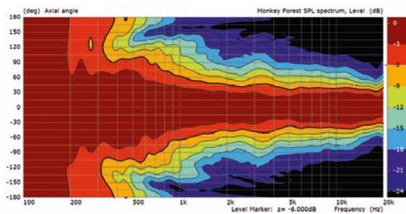
Horizontal directivity
