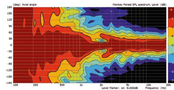
Vertical directivity
