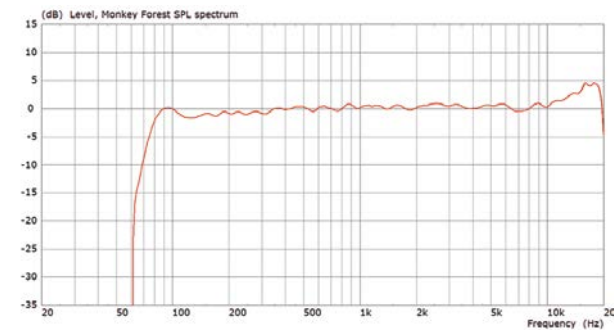
Frequency response (with controller)
