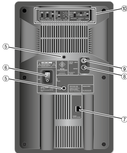
Back panel
