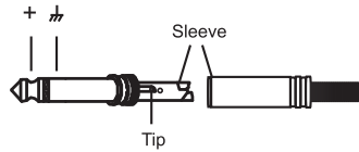
1/4" TS jack Unbalanced input/output
