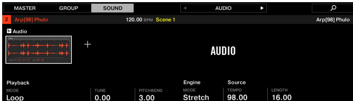
Audio Plug-in
