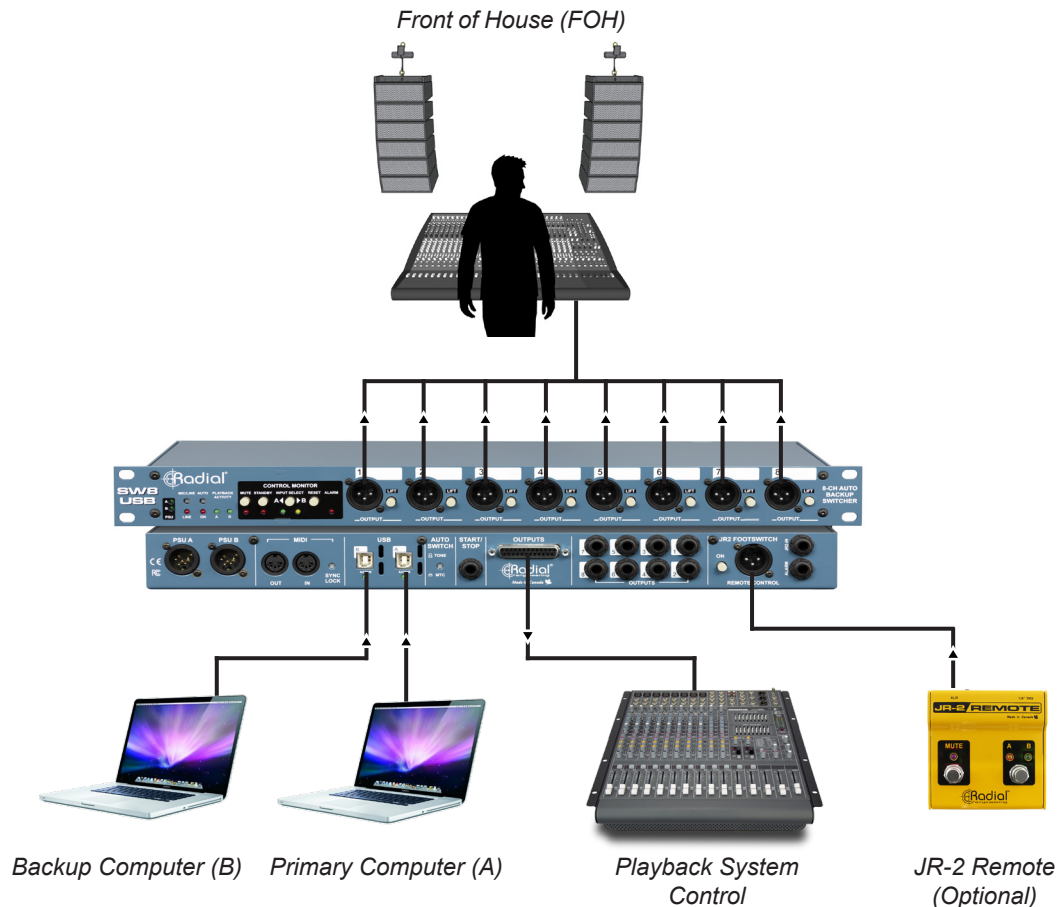
Typical stage setup for playing backing tracks through the SW8-USB
