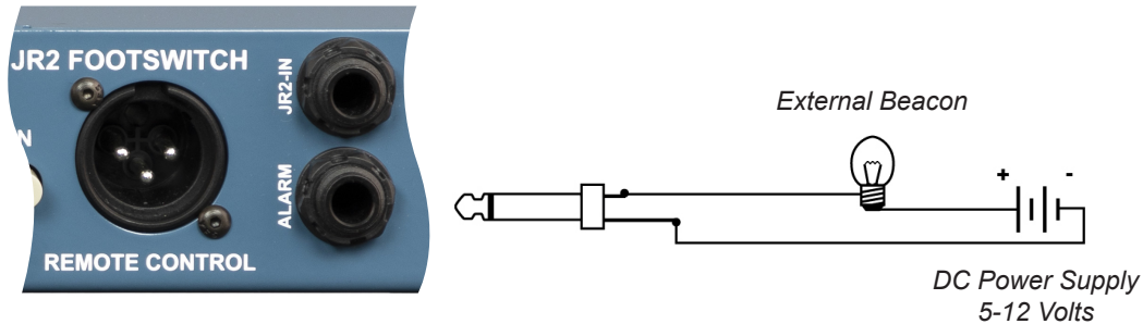
Using the ALARM output to trigger an external device
