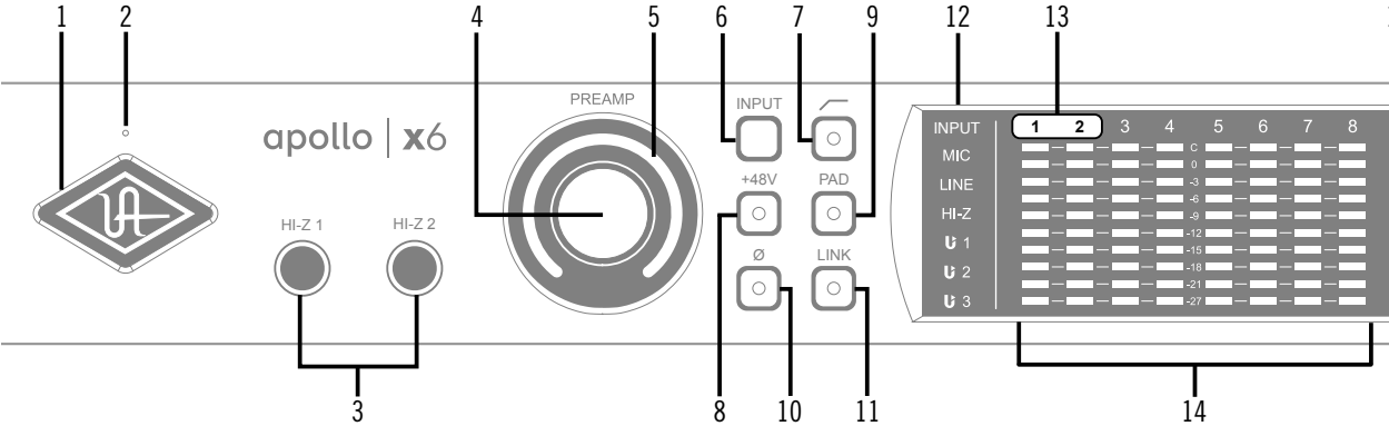
Apollo x6 front panel (left portion)
